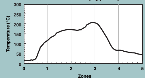
IR Reflow Profile (Typical)
